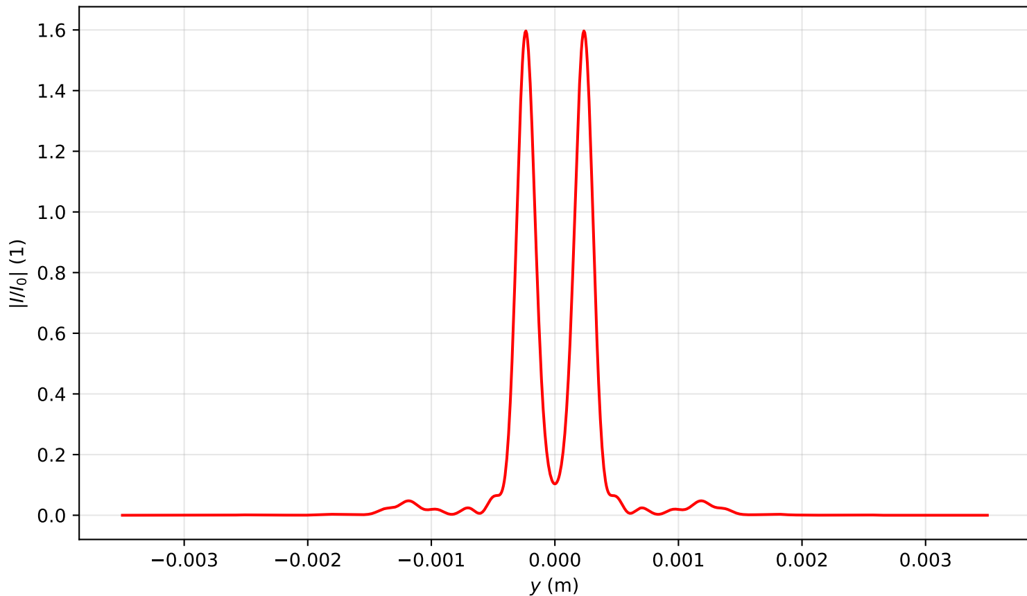
Intensity profile I(x=0, y, z=1.672)/I_0 , P_{in}=3.5P_{cr} , artificial time
